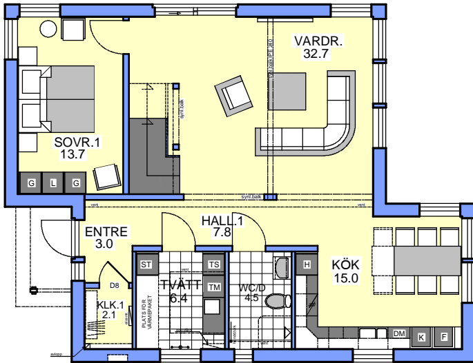
ENTRÉPLAN BOA 87.5 m 2 TOT. BOA 175.0 m 2
